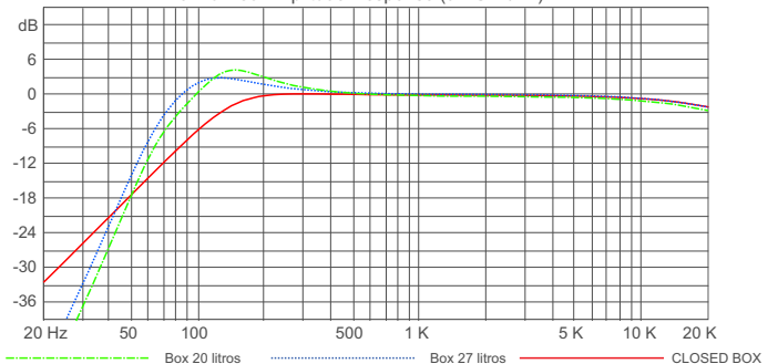
Normalized Amplitude Response (dB-SPL/Hz)
